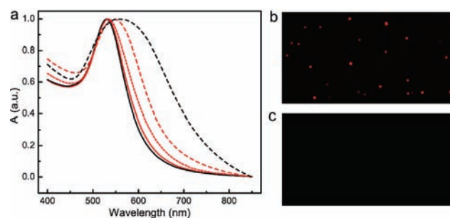
Figure 3. (a) UV–vis spectra of the amphiphilic nanocrystals in chloroform and the vesicles in aqueous media: Au@PEG/PMMA (black solid line), vesicles of Au@PEG/PMMA (black dashed line), Au@PEG/PMMAVP containing 25% 4VP in the hydrophobic brush (red solid line), vesicles of Au@PEG/PMMAVP at pH 7.0 (red dashed line), and the disassembled vesicles of Au@PEG/PMMAVP at pH 5.0 (red dot line). (b, c) Dark-field microscope images of the vesicles of Au@PEG/PMMAVP at (b) pH 7.0 and (c) pH 5.0.
